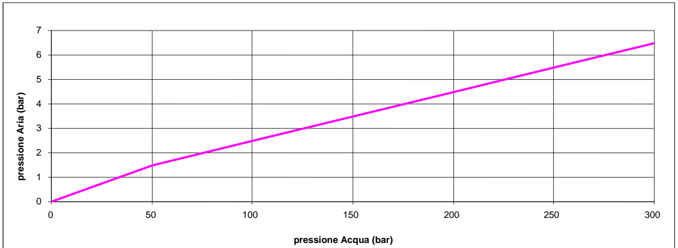
DIAGRAMMA PRESSIONI ARIA – ACQUA AIR – WATER PRESSURE CHART
